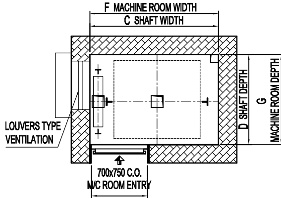
Cross Sectional Plan Of Machine Room
