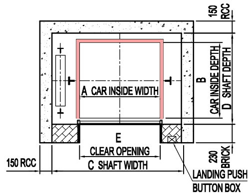
Cross Sectional Plan Of Elevator Shaft
