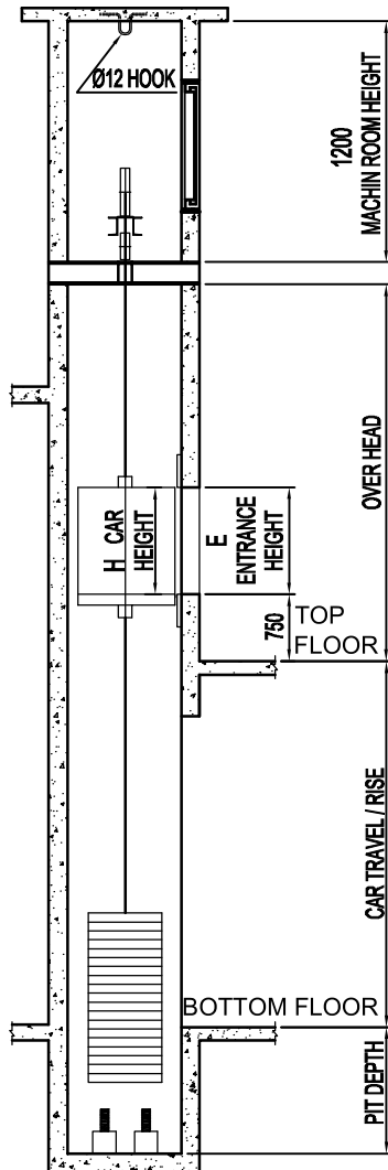
Sectional Elevation Of Elevator Shaft
